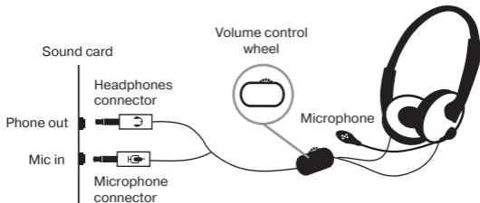
Fig. 1. Connection diagram
